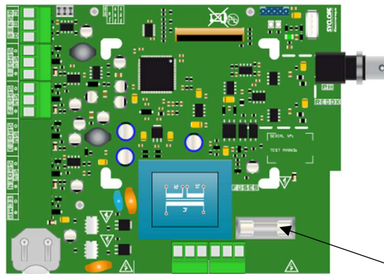
Glass Fuse 5x20 250mA Time-lag
